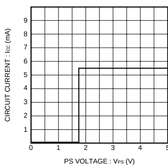
Fig.8 PS Threshold voltage
